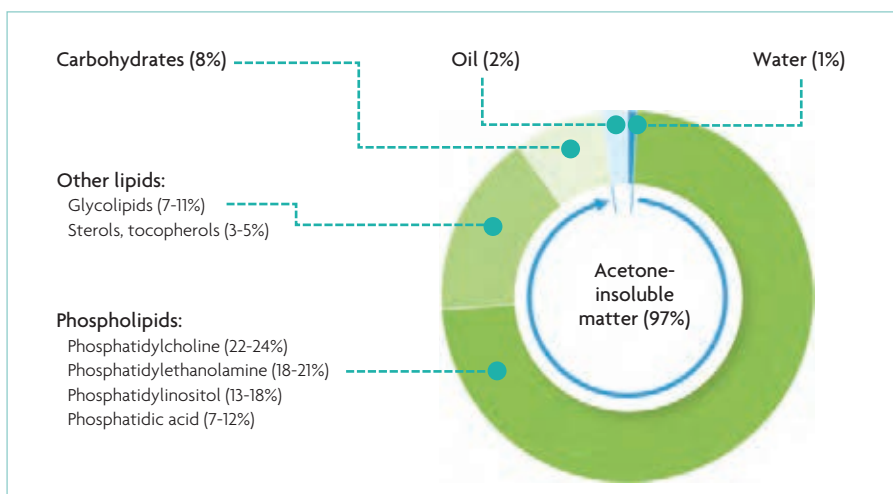
Fig. 1. The constituents of deoiled lecithin.
